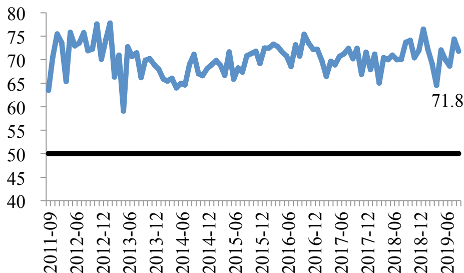
Figure 12 Industry Competitiveness
