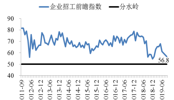
Figure 11 Recruitment Index
